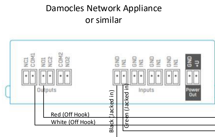
183mm cable P/N TelINF/TRRSMC6
